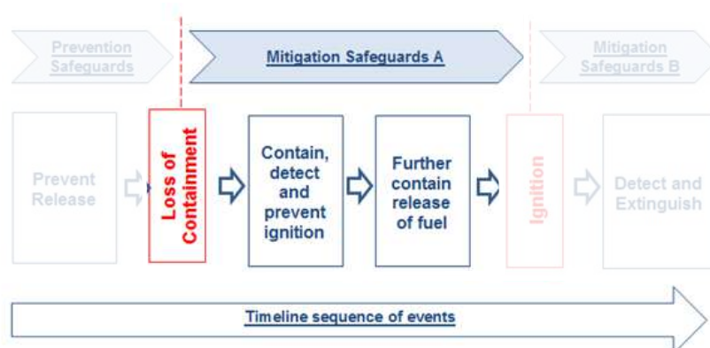
Figure 14.6 – LNG Bunkering Layers of Defence (2 nd Layer of Defence – Mitigation A)
