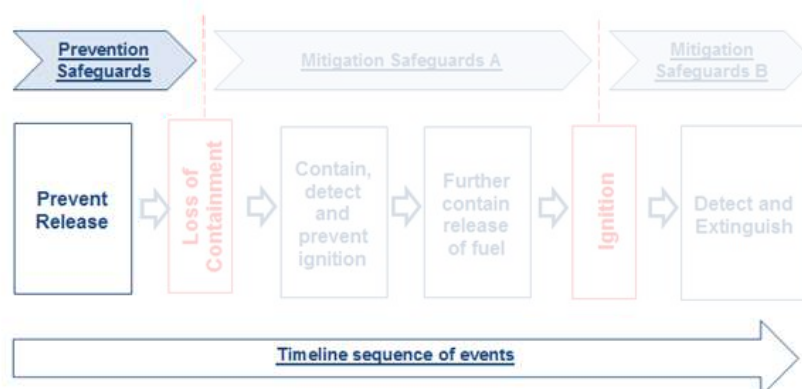
Figure 14.5 – LNG Bunkering Layers of Defence (1 st Layer of Defence - Prevention)
