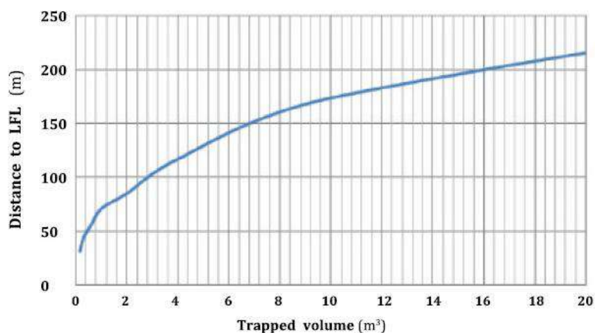
Figure 9.11 – Flammable extent with respects to volume of released LNG (reproduced from ISO 20519 figure B.3)
