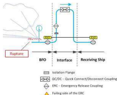
Figure 9.11 – Illustration of the trapped inventory release (between ESD and failing ERC side)
