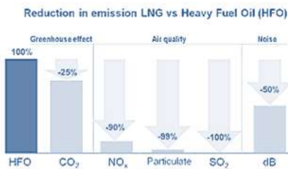
Fig.2 – Potential reduction of air emissions (relative to use of HFO). The total elimination of Particulate Matter and Sulphur dioxide is the most relevant benefit, at local level, of a switch to LNG fuel.
