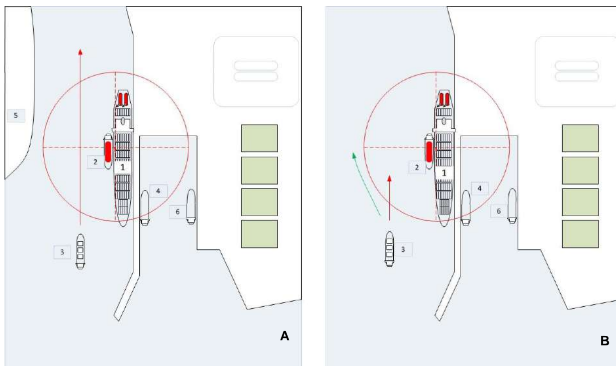
Figure 9.21 (left) and 9.22 (right) – LNG Bunkering Safety Zone implementation – Representation of two different situations where a vessels intends to cross the Safety Zone.
