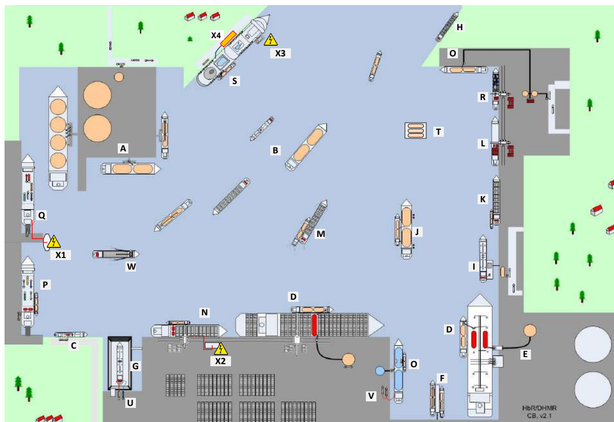
Figure 5.5 – Possible LNG bunkering activities and small-scale LNG activity within a generic layout of a Port
