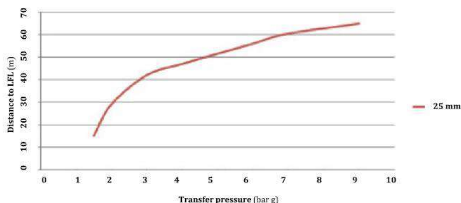
Figure 9.10 – Flammable extent with respects to pressure at LNG release point (reproduced from ISO 20519 figure B.4)
