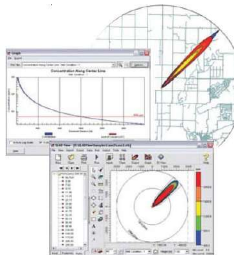
Figure 9.13 – SLAB interface representation. 2D dispersion (SLAB 3D commercial suite already available with improved visualization options)
