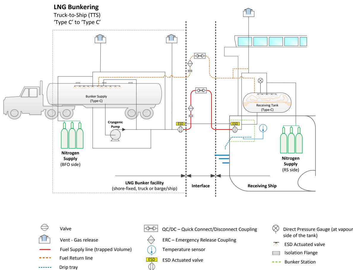
Figure 12.9 – TTS Bunkering – single line diagram for generic representation
