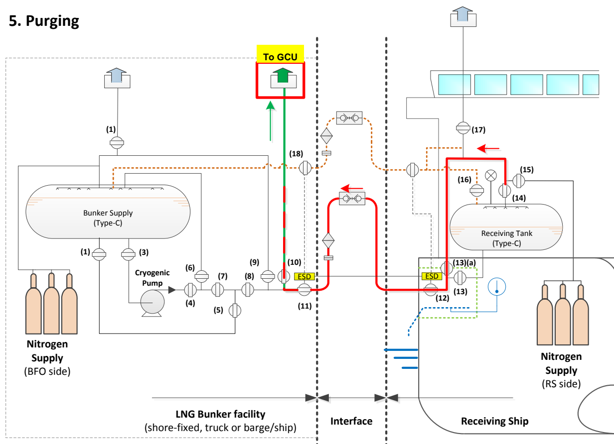
Figure 12.23 – Generic LNG Bunkering arrangement – Step 5 – Purging
