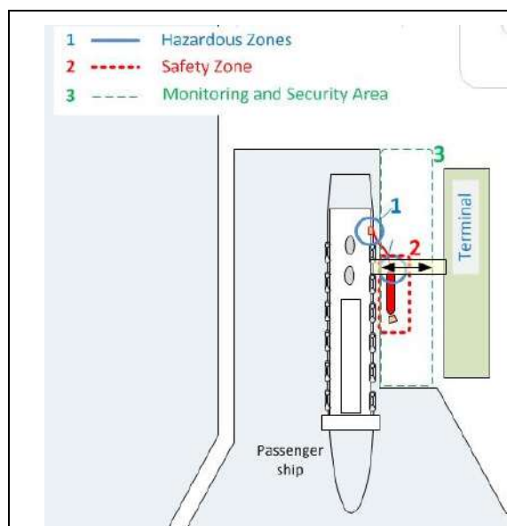
Figure 11.3 – SIMOPS and Control Zones (example – see considerations on SIMOPS on table 11.3) – passenger ship generic case – passenger embarkation/disembarkation during LNG fuelling
