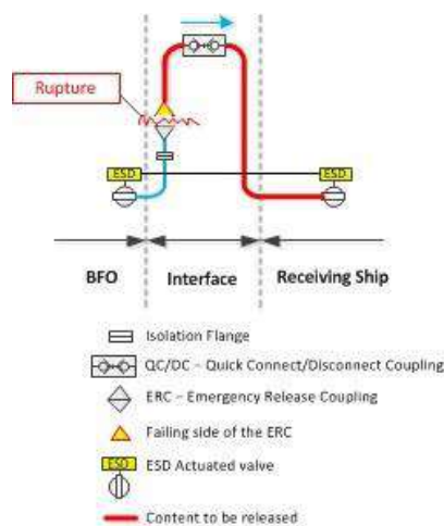
Figure 9.10 – Illustration of the trapped inventory release (between ESD and failing ERC side)
