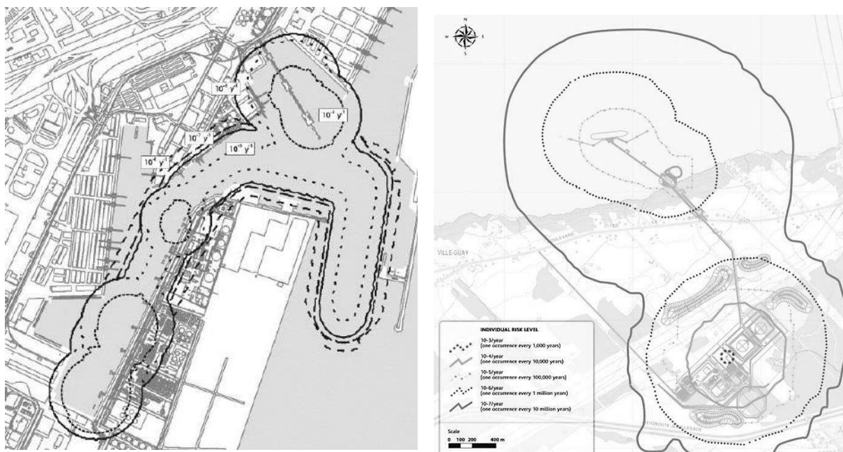
Figure 8.13 and 8.14 – Individual Risk contours combined in a port area. It can be seen how higher inner individual risk curves are “concentrical” to the berthing areas, revealing harm potential from activities taking place in these locations (LNG bunkering could be one of these activities, contribution to the composed IR combined shape).
