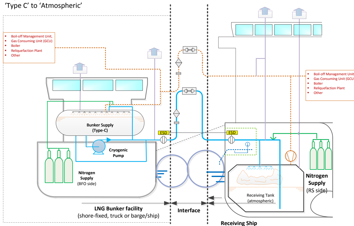
Figure 12.14 – TTS Bunkering – single line diagram for generic representation
