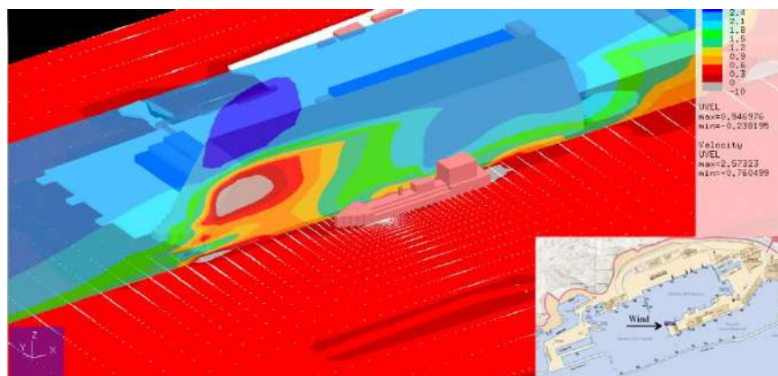
Figure 9.14 – CFD representation of an LNG cloud release, following a modelled STS bunkering. Local wind and turbulence effects are modelled, providing a more accurate analysis of non-linear situations. To be noted the effect of the inter-ship space, where LNG cloud dispersion is bounded by the ship's shape, leading to a dispersion progression which is far from regular. (courtesy: LR/ Port of Marseille)
