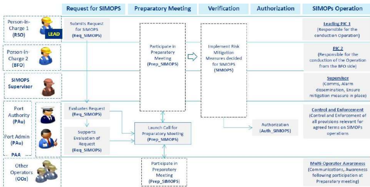
Figure 11.7 –SIMOPS in LNG Bunkering Operations – Recommended Operational Diagram
