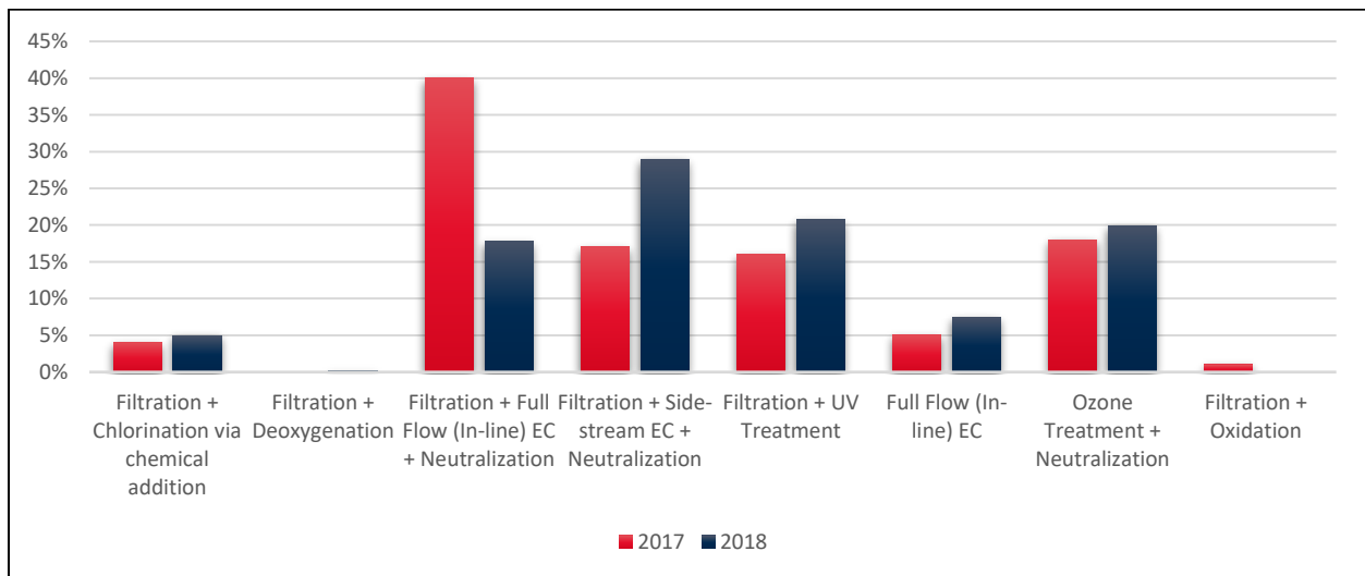
Figure 8 BWMS Technology Types (2017 vs 2018)
