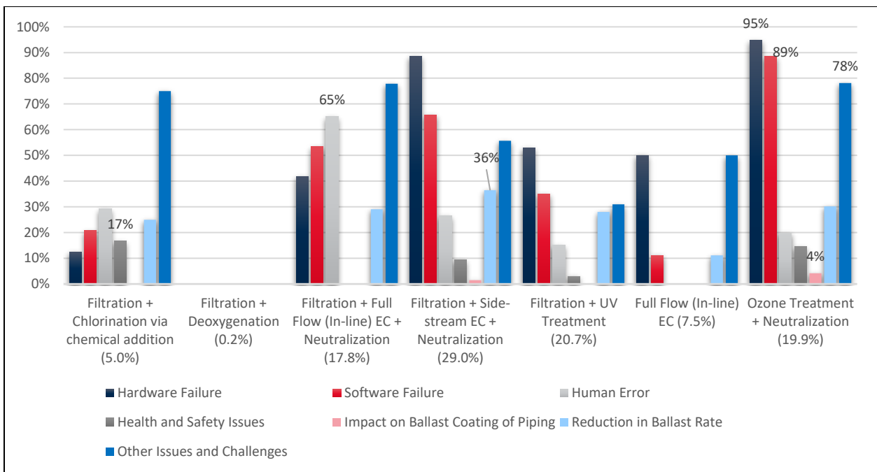
Figure 4 In-Operation Concerns Reported
