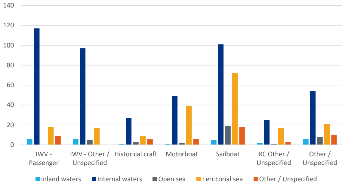
Figure 7.9: Distribution by location of marine casualties and incidents per other ship type for 2014-2019
