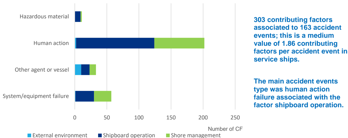
Figure 6.11: Relationship between accident events and the contributing factors in service ships for 2014-2019
