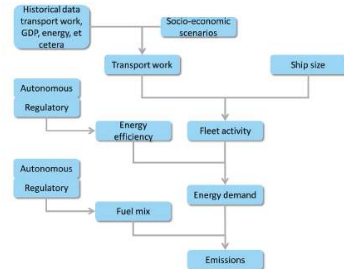
Figure 23 – Graphical representation of methodology to develop emission projections
