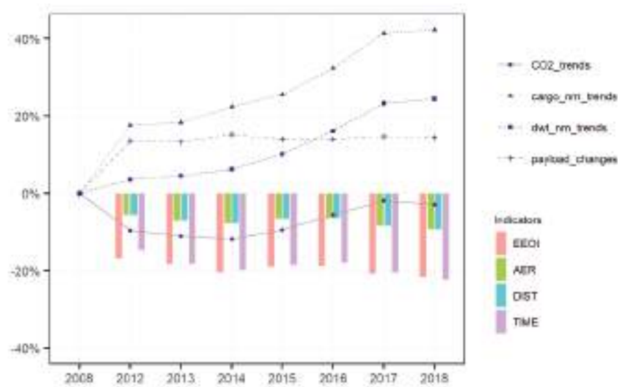
Figure 15 – Percentage changes in individual based carbon intensity of international shipping (vessel-based)
