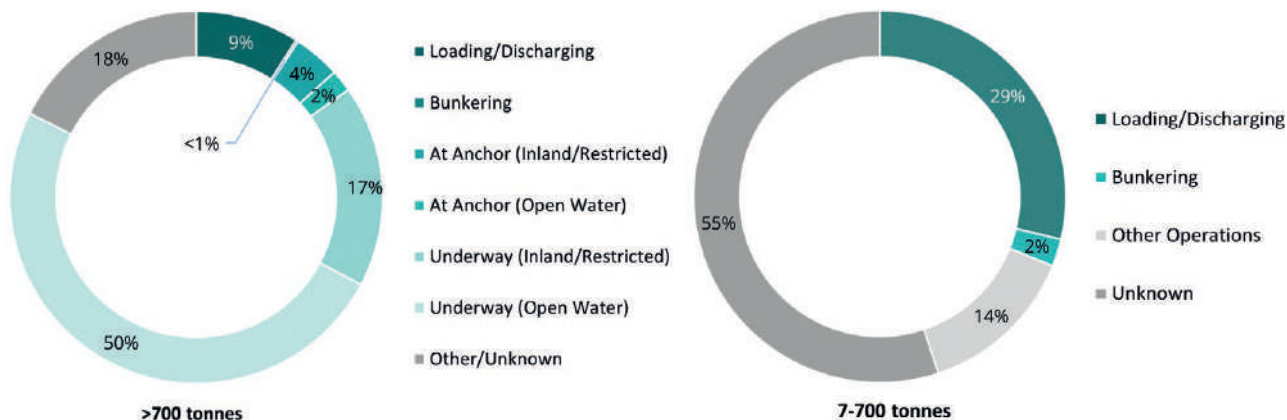
Figure 12: Number of tanker spills by operation at time of incident, 1970-2021
