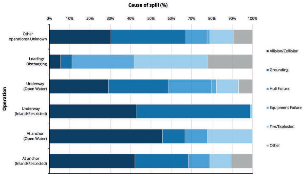
Figure 13: Number of tanker spills >700 tonnes by operation at time of incident and primary cause of spill, 1970-2021
