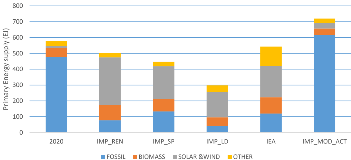
Figure 6: 2050 primary energy by type and scenario. NB: other comprises sources such as hydro, nuclear etc. and hydrogen as a secondary fuel will be captured within 'fossil' or 'solar & wind' depending on whether it is grey, blue or green.
