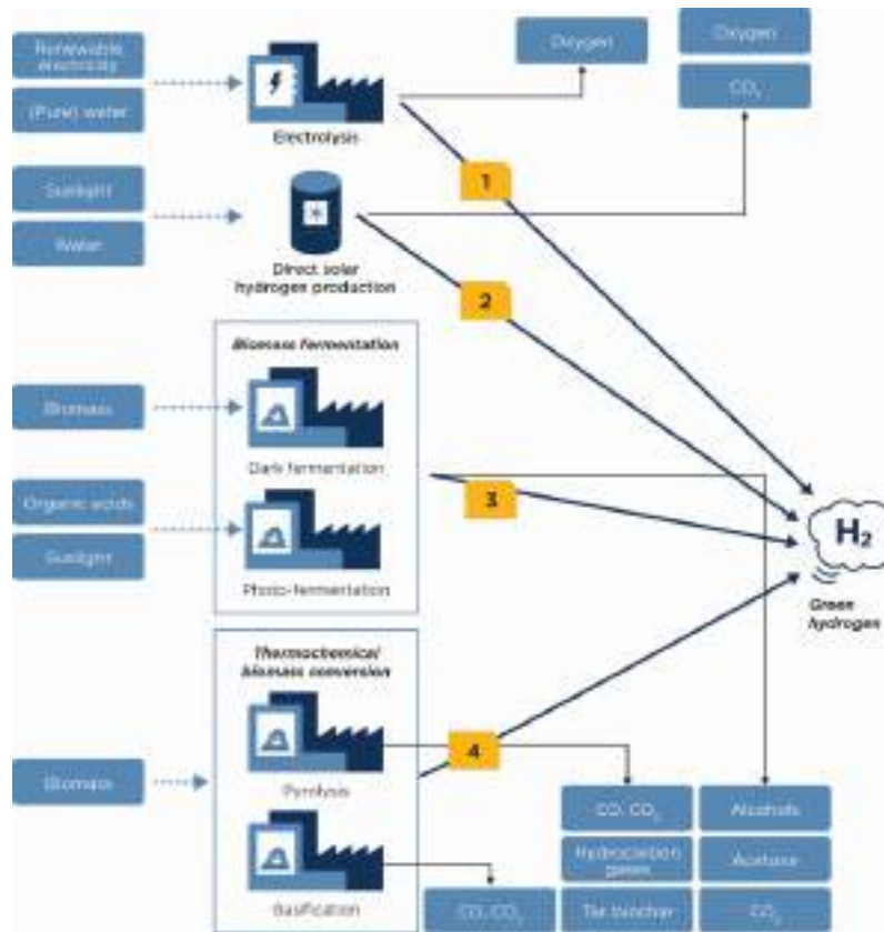
Figure 1. Production pathways for green hydrogen.
