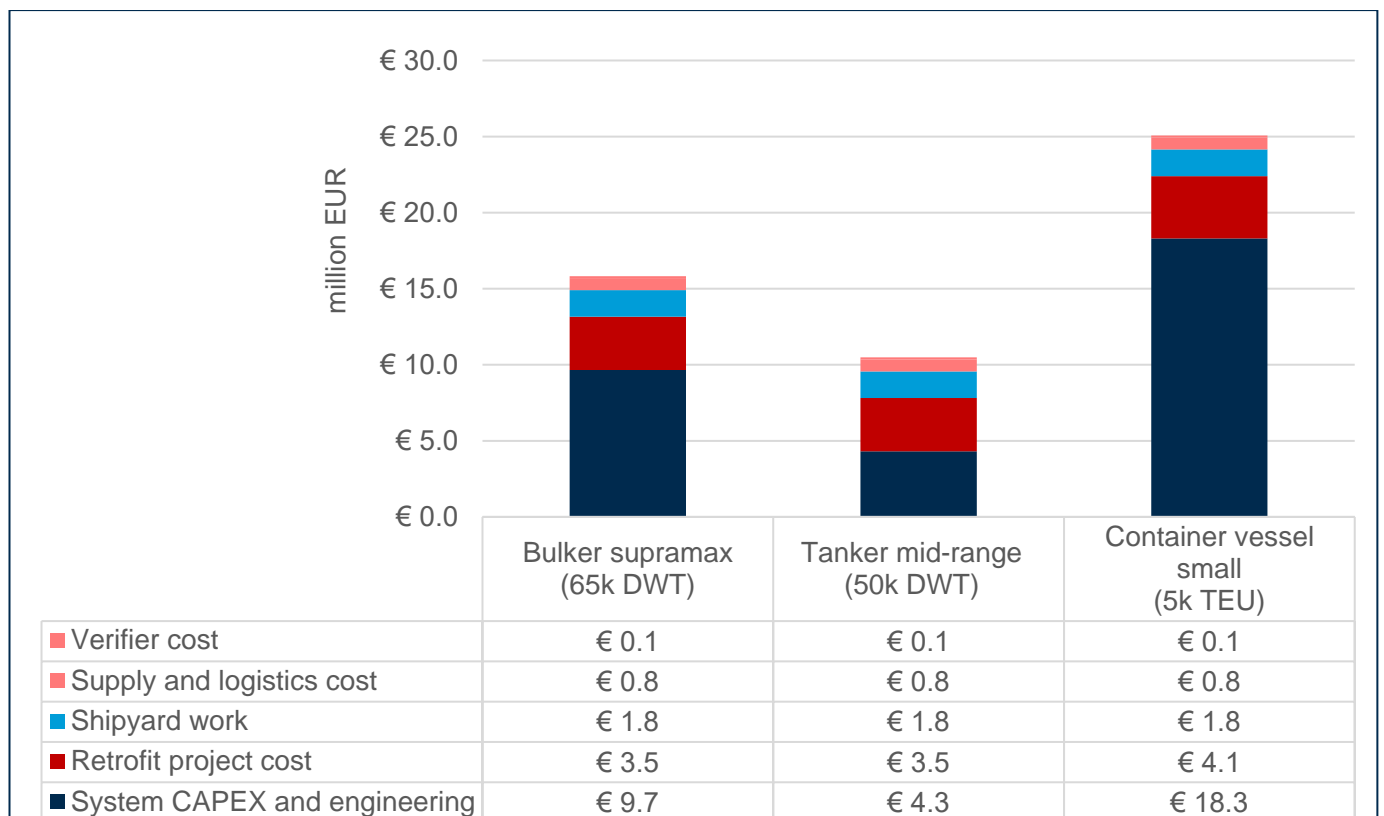
Figure 18. Total cost of retrofitting (million EUR) conventional fuel to hydrogen ICE system
