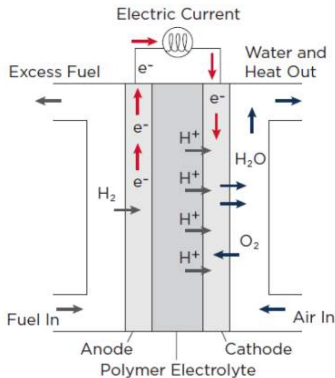
Figure 11. A typical Proton Exchange Membrane (PEM) Fuel Cell (ABS, Sustainability Whitepaper, Hydrogen as Marine Fuel, 2021)
