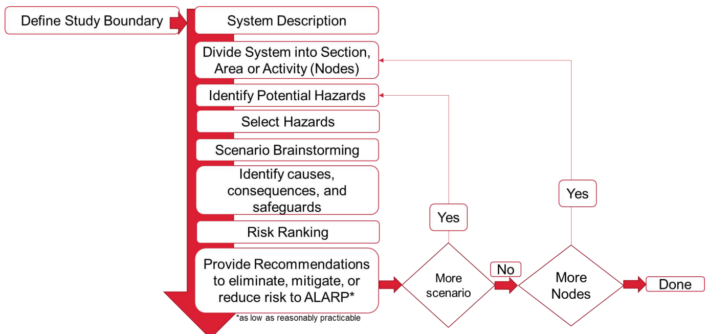
Figure 27. HAZID Process
