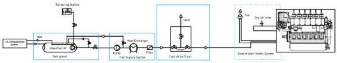
Figure 7. Schematic onboard hydrogen installation of the FSS for a 2-stroke Diesel-cycle hydrogen engine
